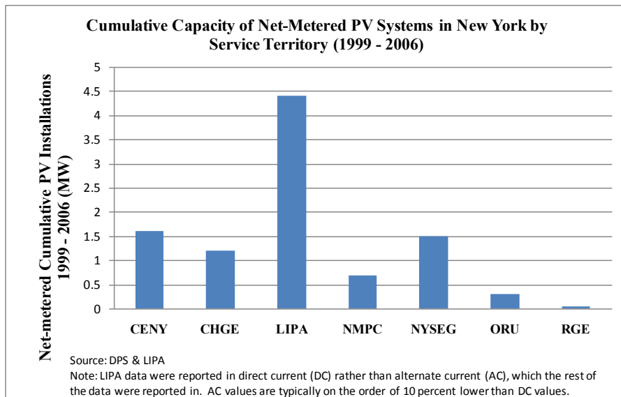
Figure 9. 1999-2006 Cumulative Capacity of Customer-Sited, Net-Metered Solar-PV Systems by Service Territory
